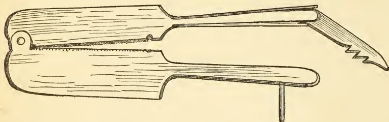
FIG. 133.— The Castrating Clams of Messrs. Burgess, Willows, & Co.
